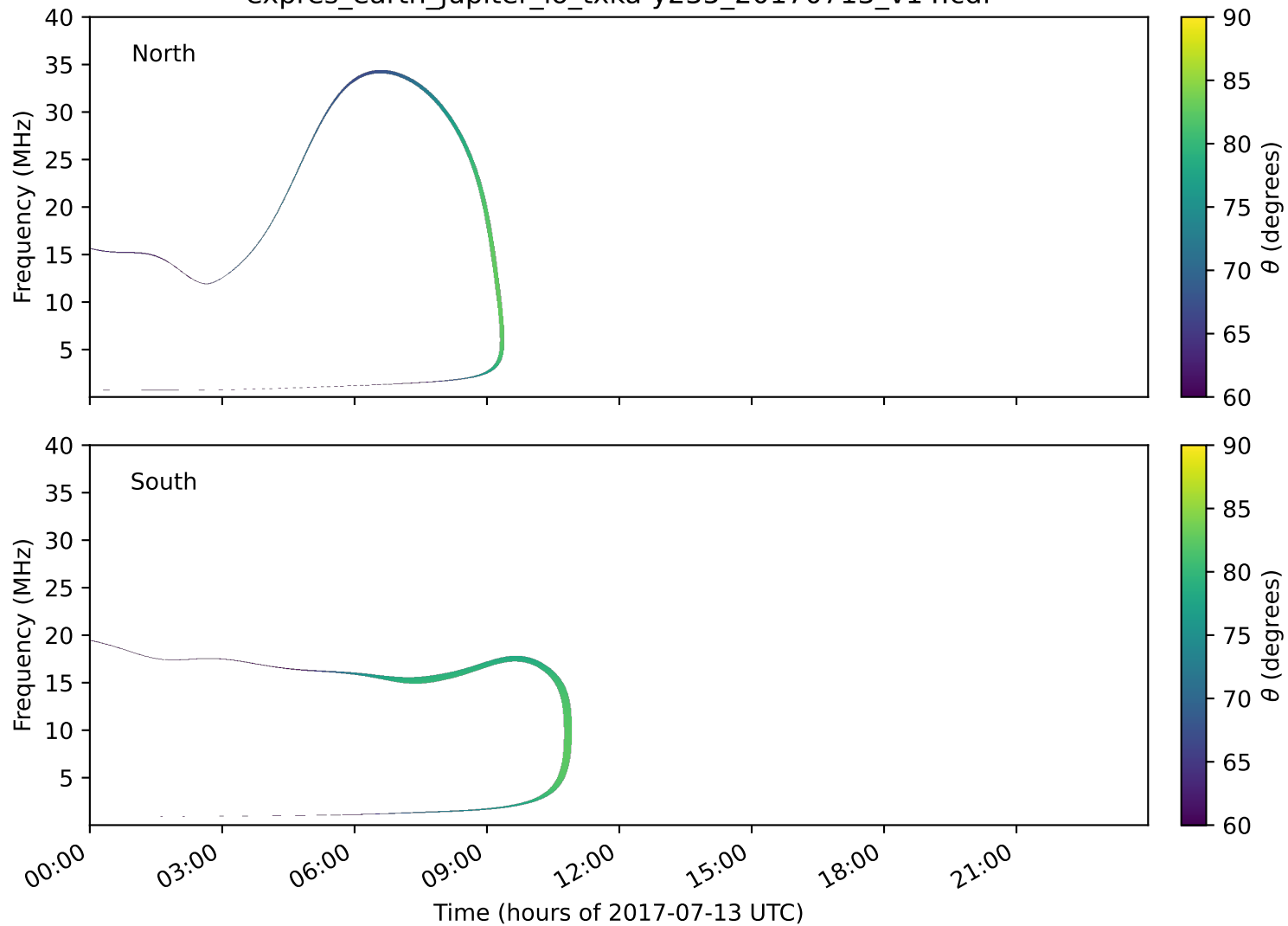
expres_earth_jupiter_io_txka-y235_20170713_v14.cdf
