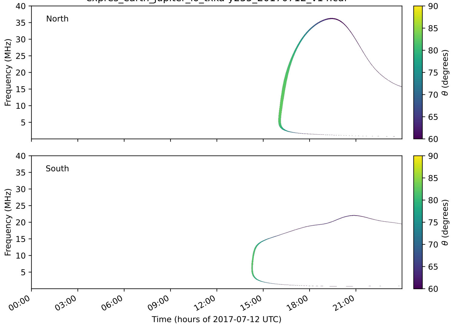
expres_earth_jupiter_io_txka-y235_20170712_v14.cdf
