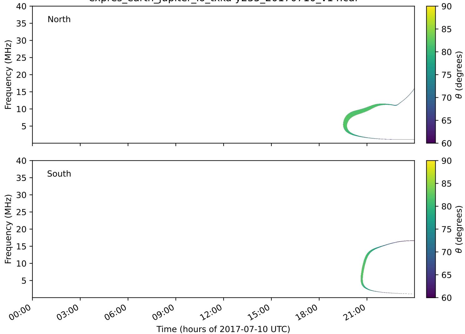
expres_earth_jupiter_io_txka-y235_20170710_v14.cdf
