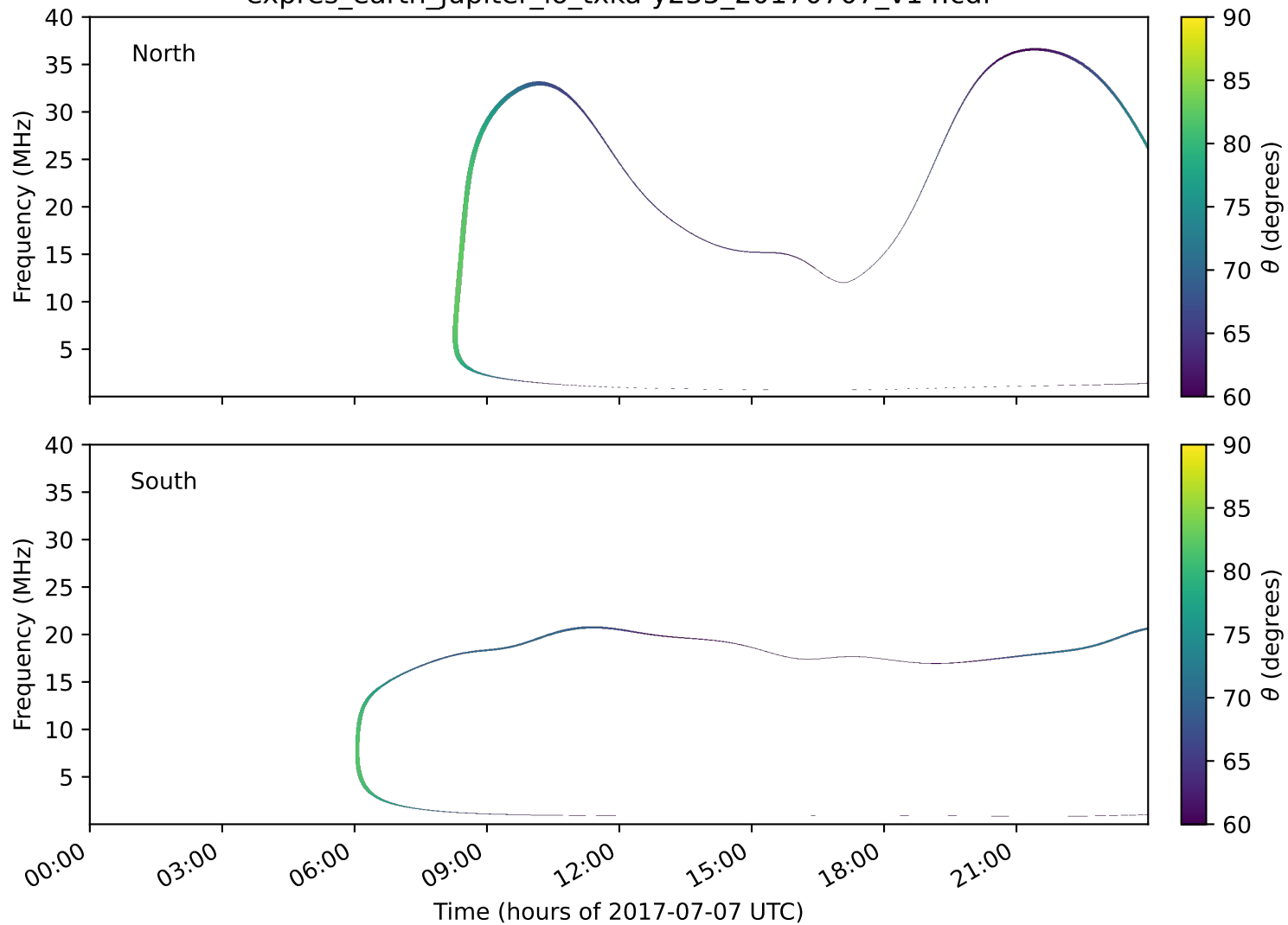
expres_earth_jupiter_io_txka-y235_20170707_v14.cdf
