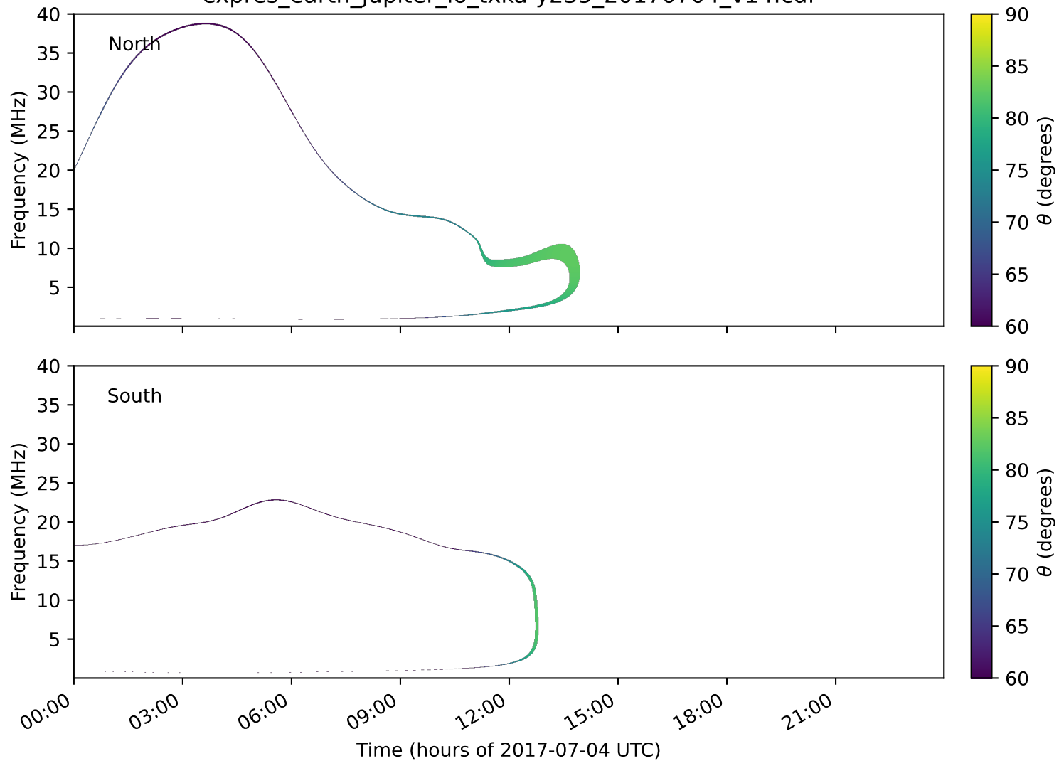
expres_earth_jupiter_io_txka-y235_20170704_v14.cdf
