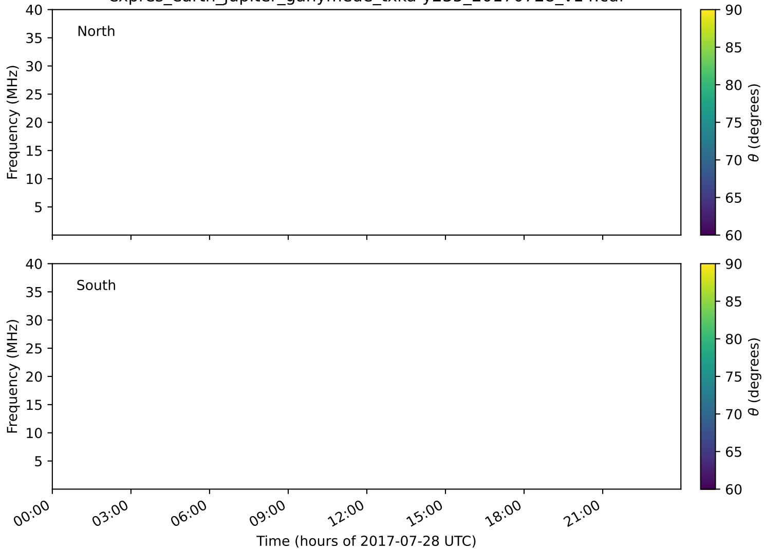
expres_earth_jupiter_ganymede_txka-y235_20170728_v14.cdf
