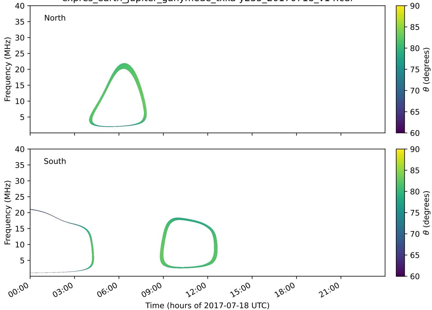
expres_earth_jupiter_ganymede_txka-y235_20170718_v14.cdf
