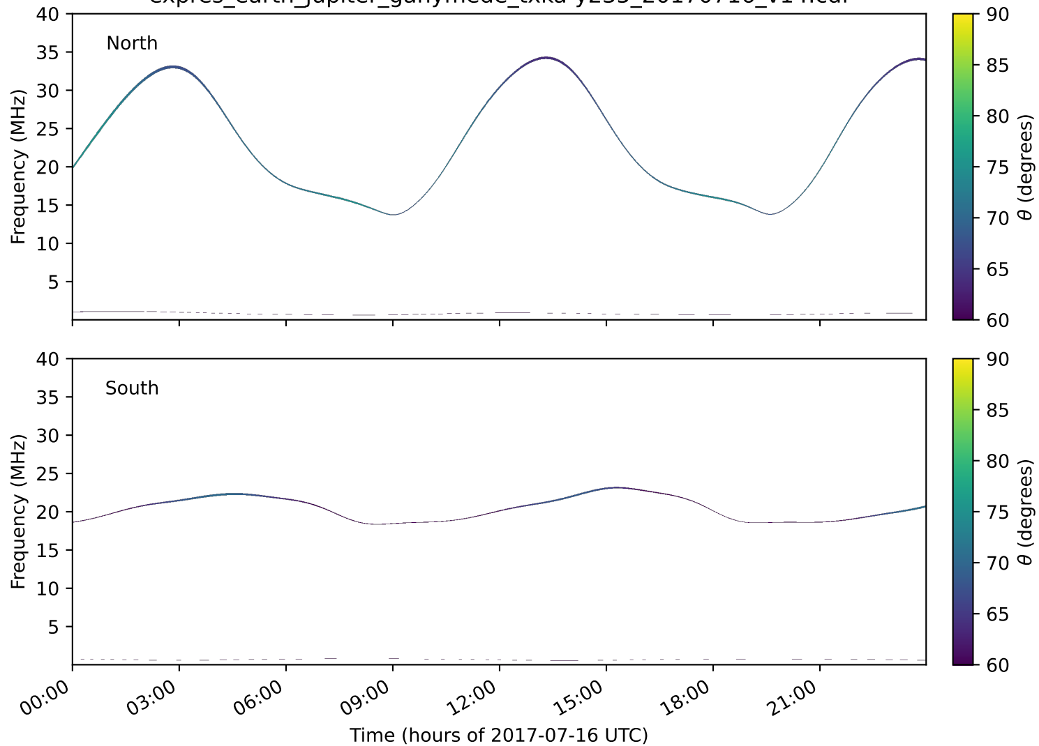
expres_earth_jupiter_ganymede_txka-y235_20170716_v14.cdf
