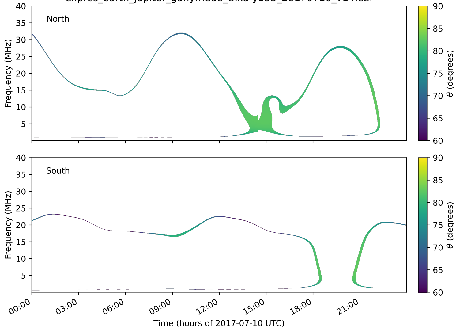
expres_earth_jupiter_ganymede_txka-y235_20170710_v14.cdf
