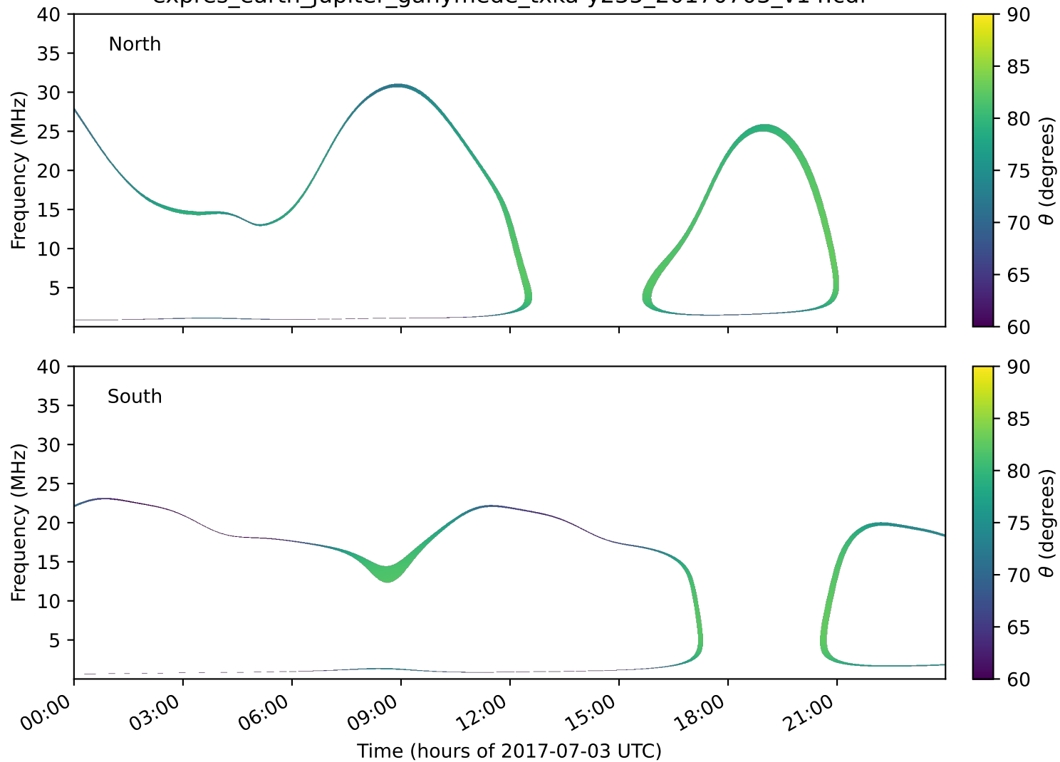
expres_earth_jupiter_ganymede_txka-y235_20170703_v14.cdf
