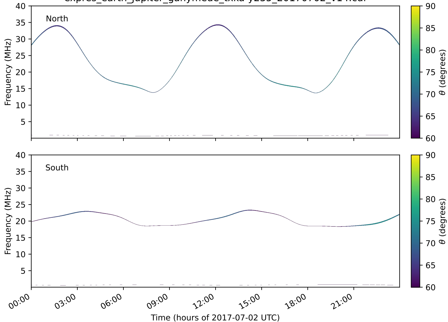
expres_earth_jupiter_ganymede_txka-y235_20170702_v14.cdf
