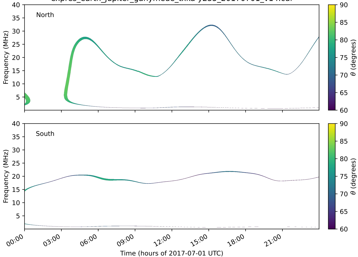
expres_earth_jupiter_ganymede_txka-y235_20170701_v14.cdf
