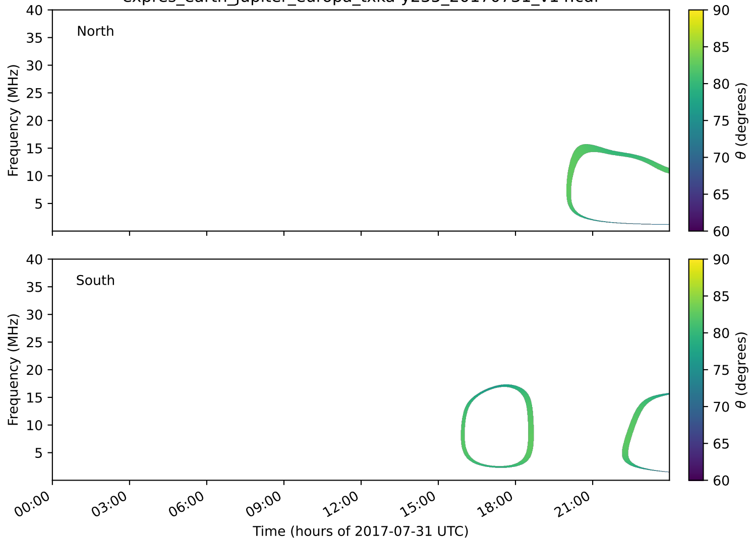
expres_earth_jupiter_europa_txka-y235_20170731_v14.cdf
