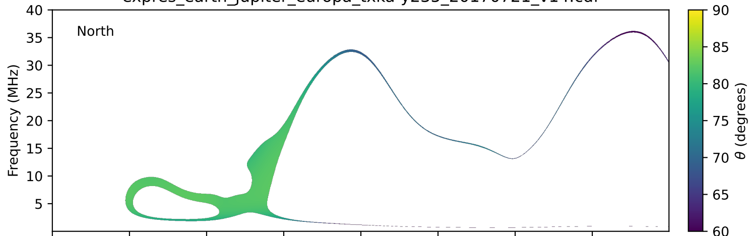
expres_earth_jupiter_europa_txka-y235_20170721_v14.cdf
