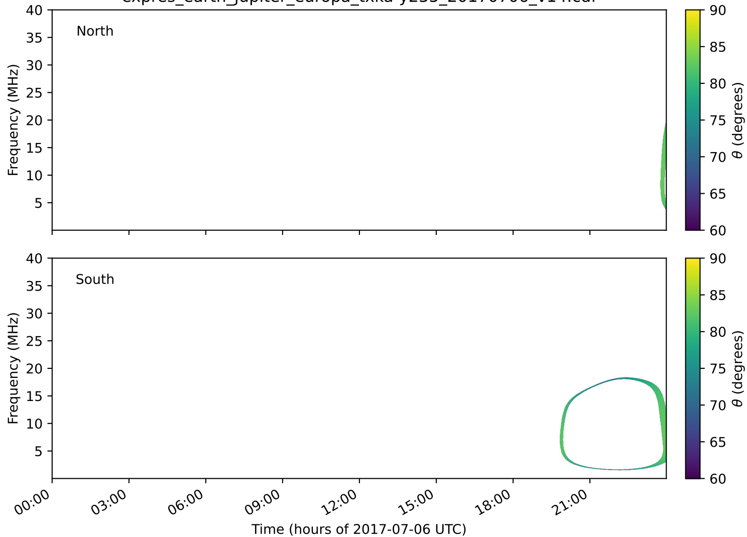
expres_earth_jupiter_europa_txka-y235_20170706_v14.cdf
