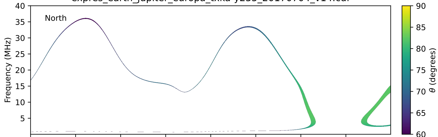
expres_earth_jupiter_europa_txka-y235_20170704_v14.cdf
