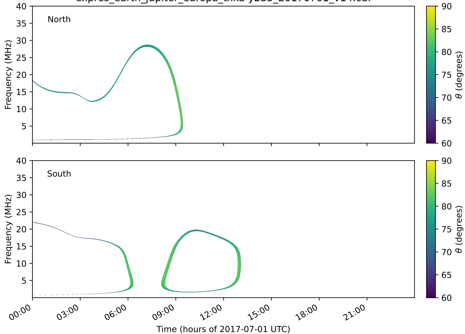
expres_earth_jupiter_europa_txka-y235_20170701_v14.cdf
