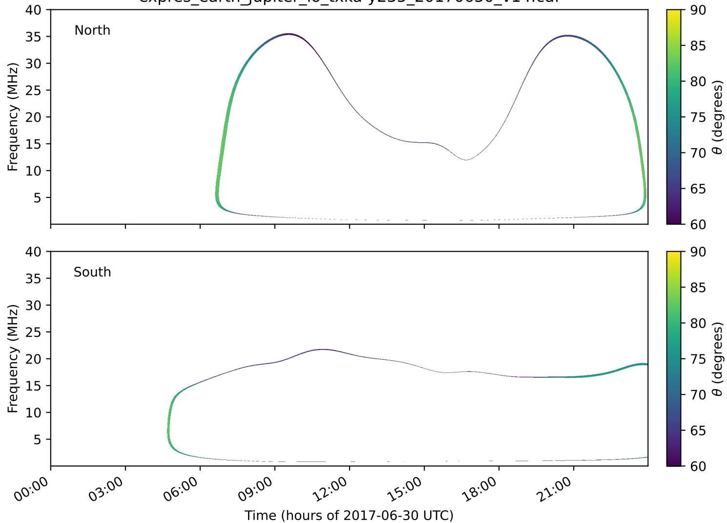
expres_earth_jupiter_io_txka-y235_20170630_v14.cdf
