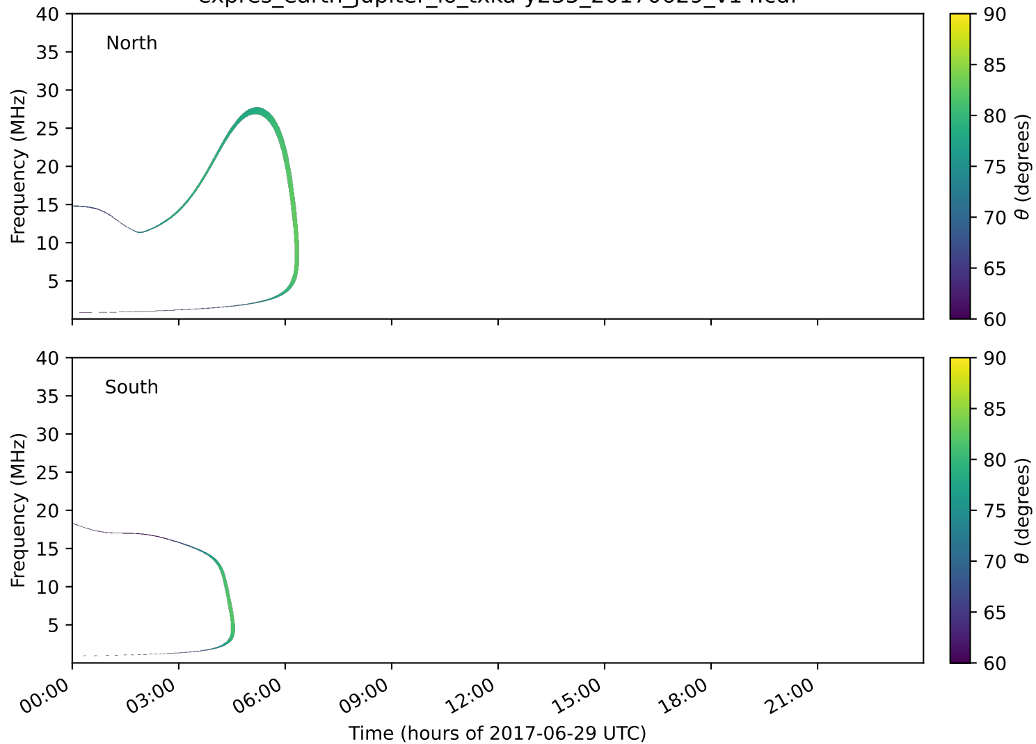
expres_earth_jupiter_io_txka-y235_20170629_v14.cdf
