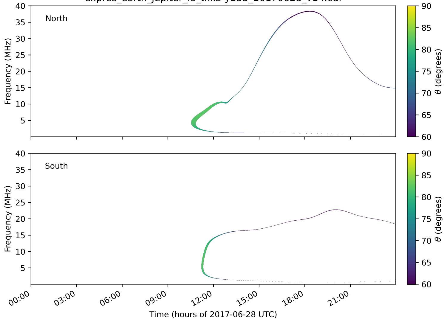
expres_earth_jupiter_io_txka-y235_20170628_v14.cdf
