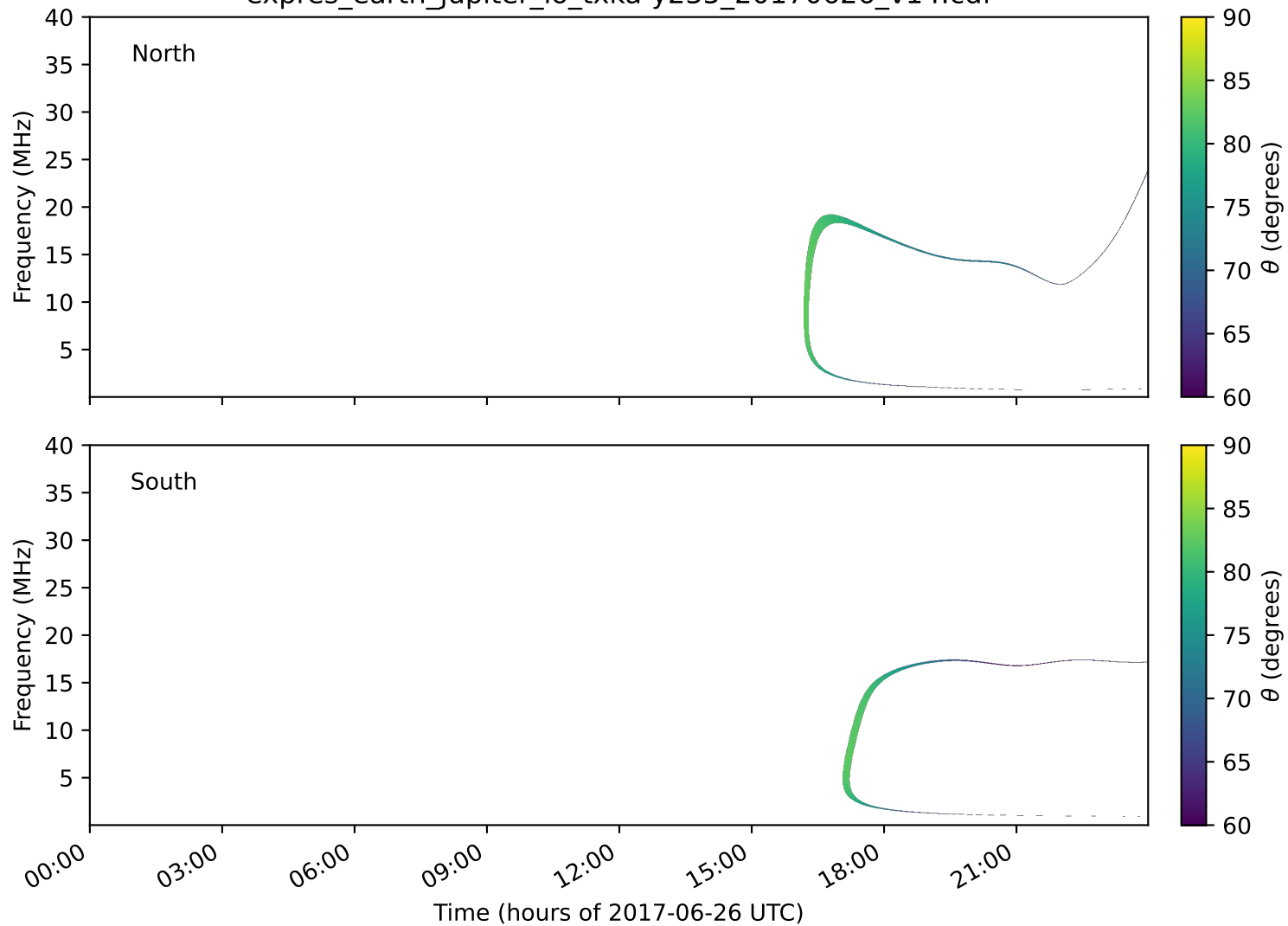
expres_earth_jupiter_io_txka-y235_20170626_v14.cdf
