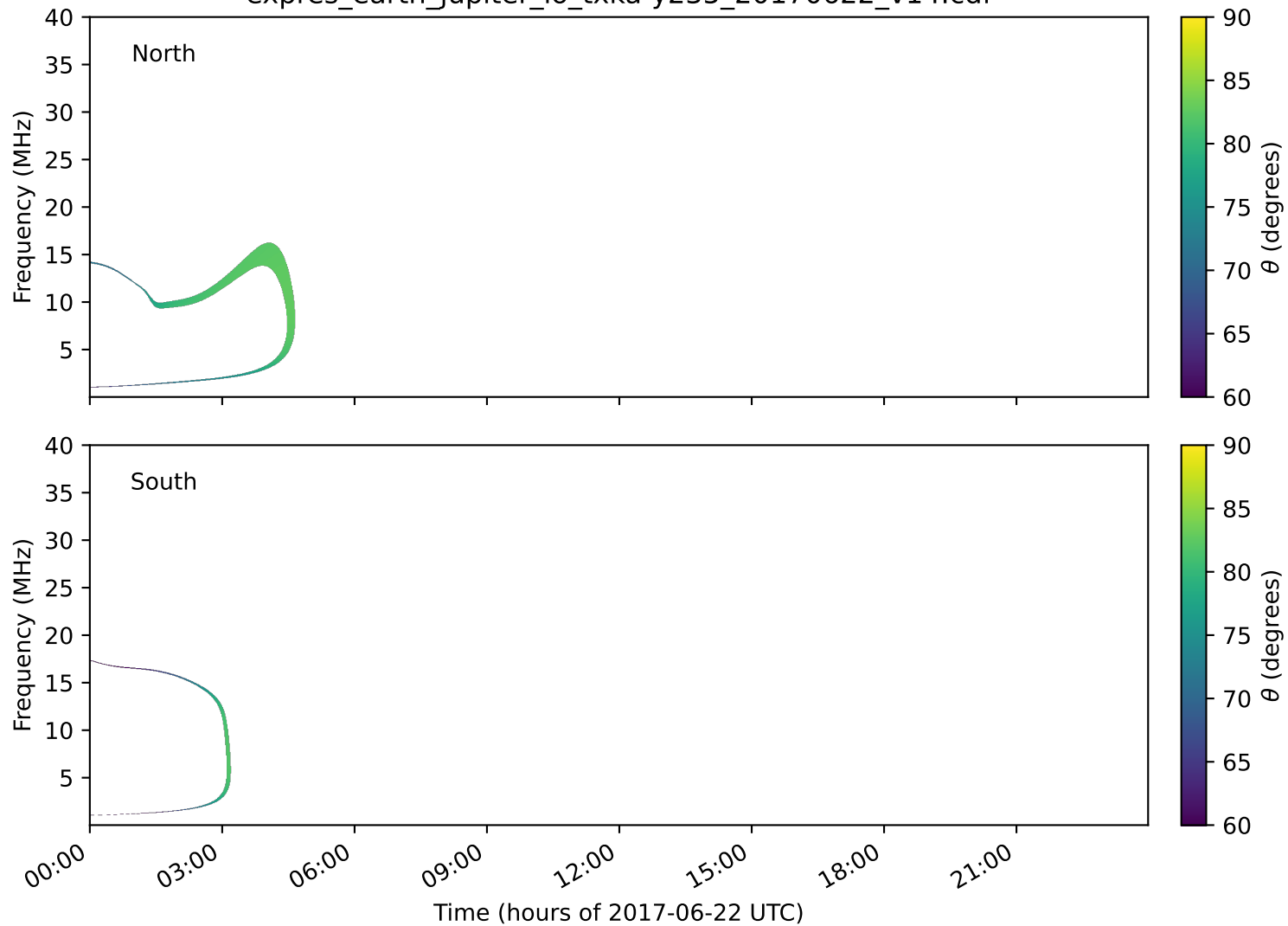
expres_earth_jupiter_io_txka-y235_20170622_v14.cdf
