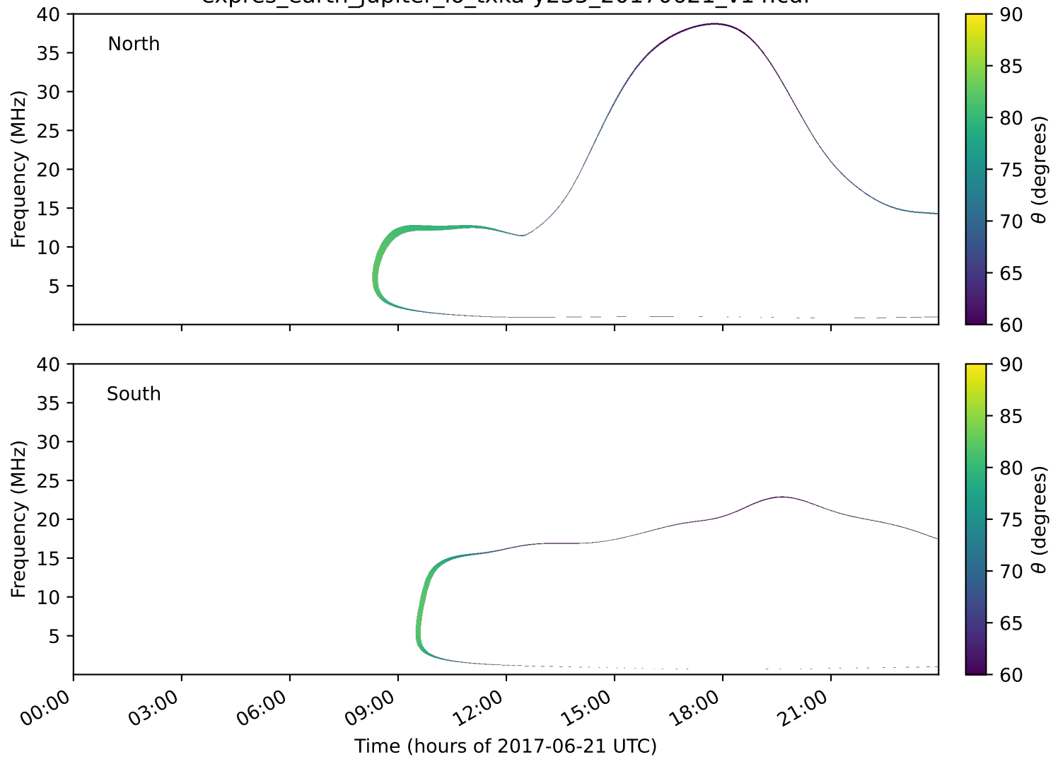
expres_earth_jupiter_io_txka-y235_20170621_v14.cdf
