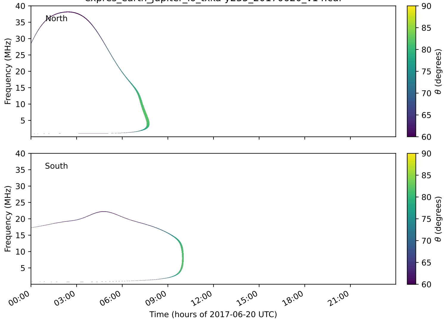
expres_earth_jupiter_io_txka-y235_20170620_v14.cdf
