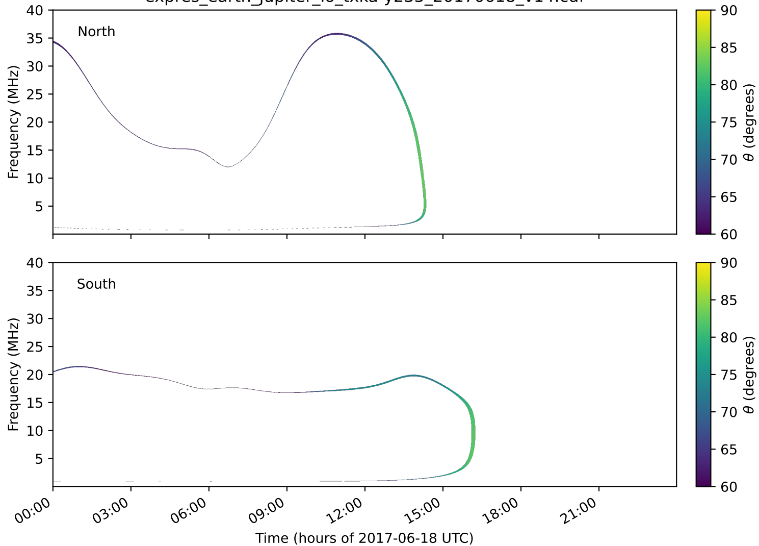
expres_earth_jupiter_io_txka-y235_20170618_v14.cdf
