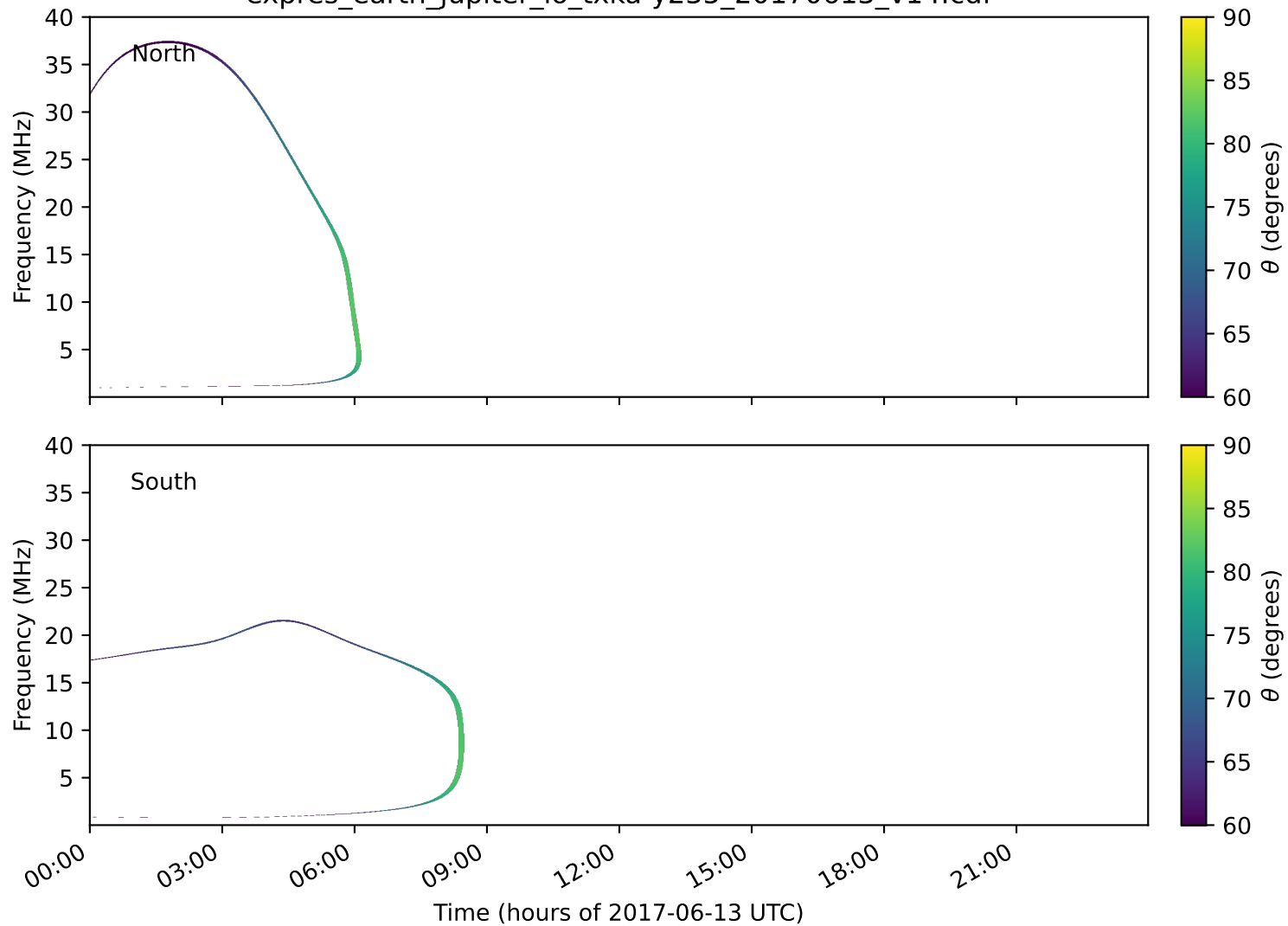
expres_earth_jupiter_io_txka-y235_20170613_v14.cdf
