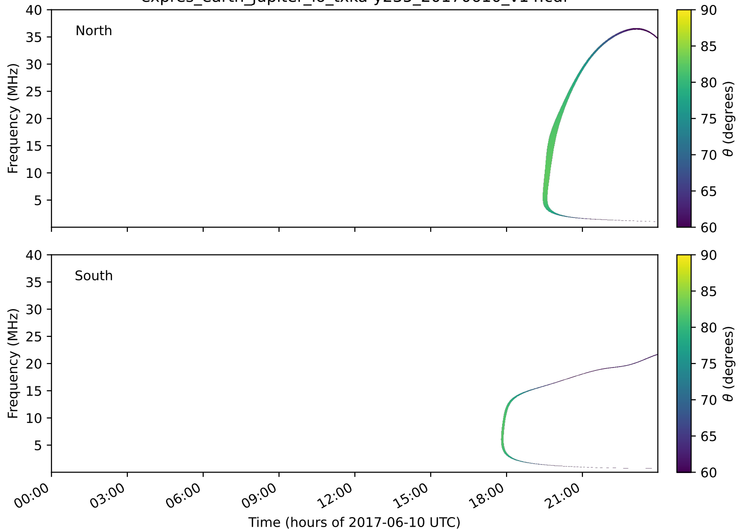
expres_earth_jupiter_io_txka-y235_20170610_v14.cdf
