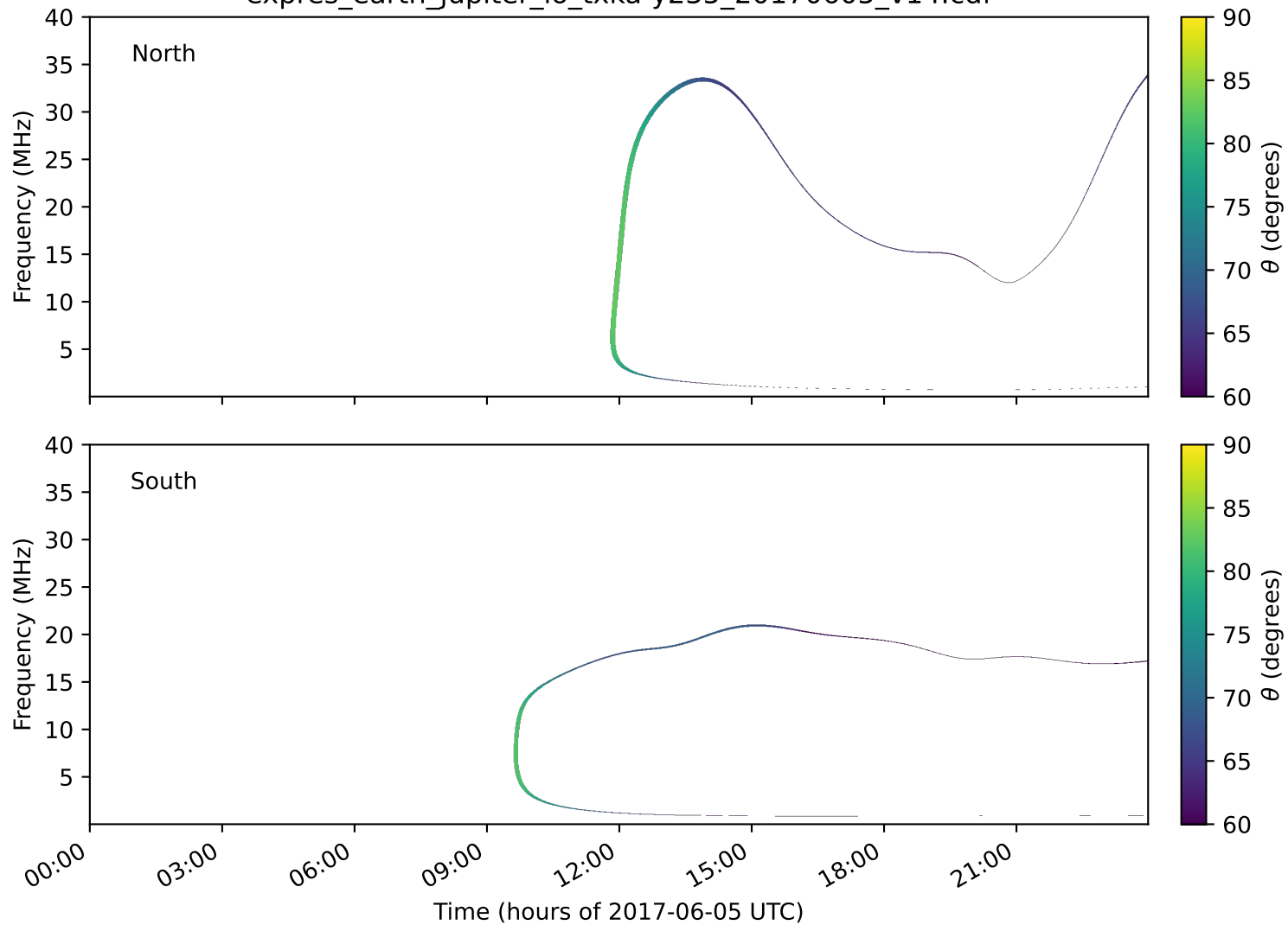
expres_earth_jupiter_io_txka-y235_20170605_v14.cdf
