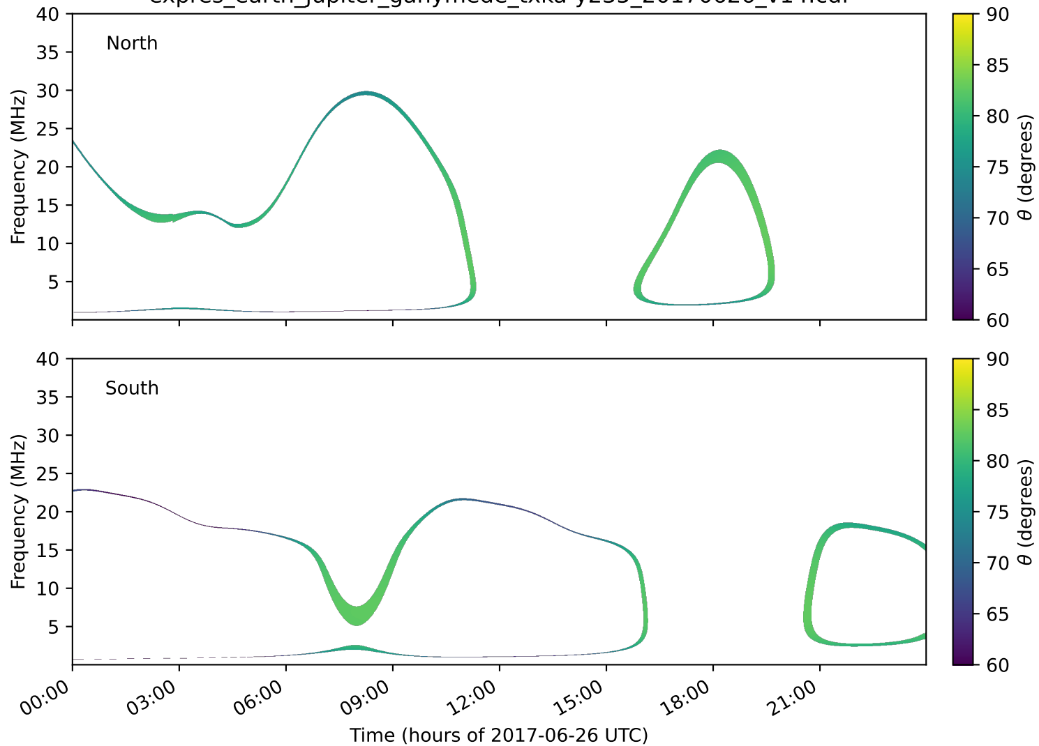
expres_earth_jupiter_ganymede_txka-y235_20170626_v14.cdf
