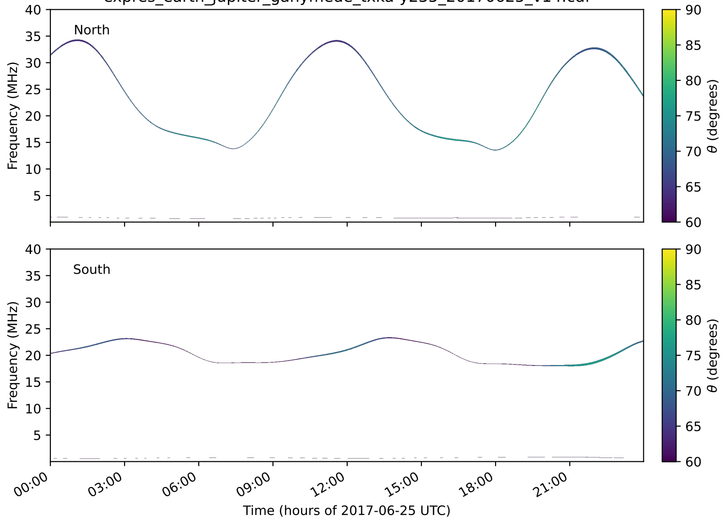
expres_earth_jupiter_ganymede_txka-y235_20170625_v14.cdf
