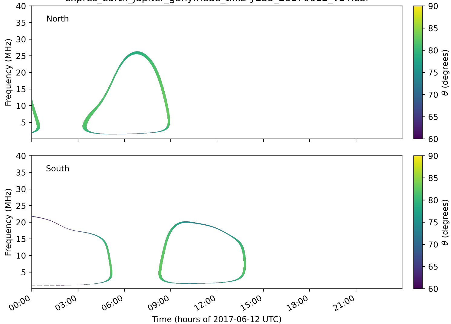
expres_earth_jupiter_ganymede_txka-y235_20170612_v14.cdf
