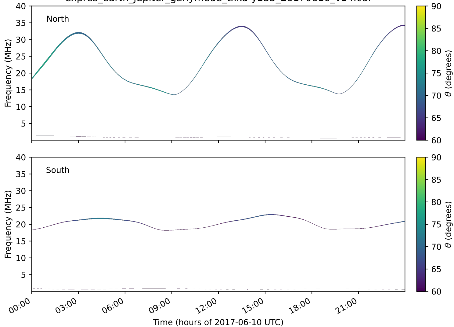
expres_earth_jupiter_ganymede_txka-y235_20170610_v14.cdf
