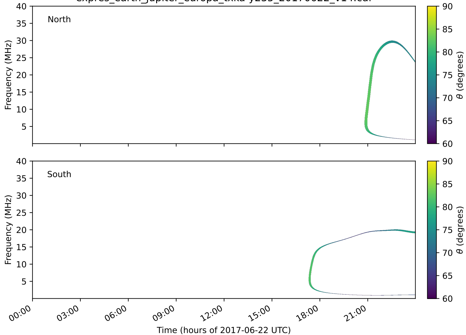
expres_earth_jupiter_europa_txka-y235_20170622_v14.cdf
