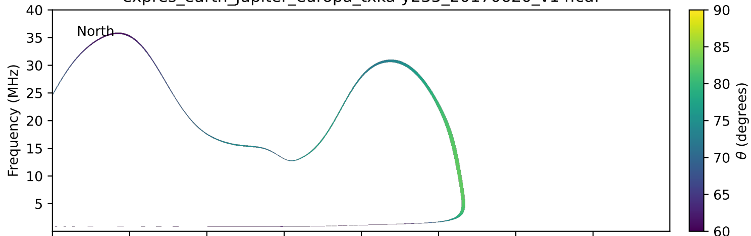
expres_earth_jupiter_europa_txka-y235_20170620_v14.cdf
