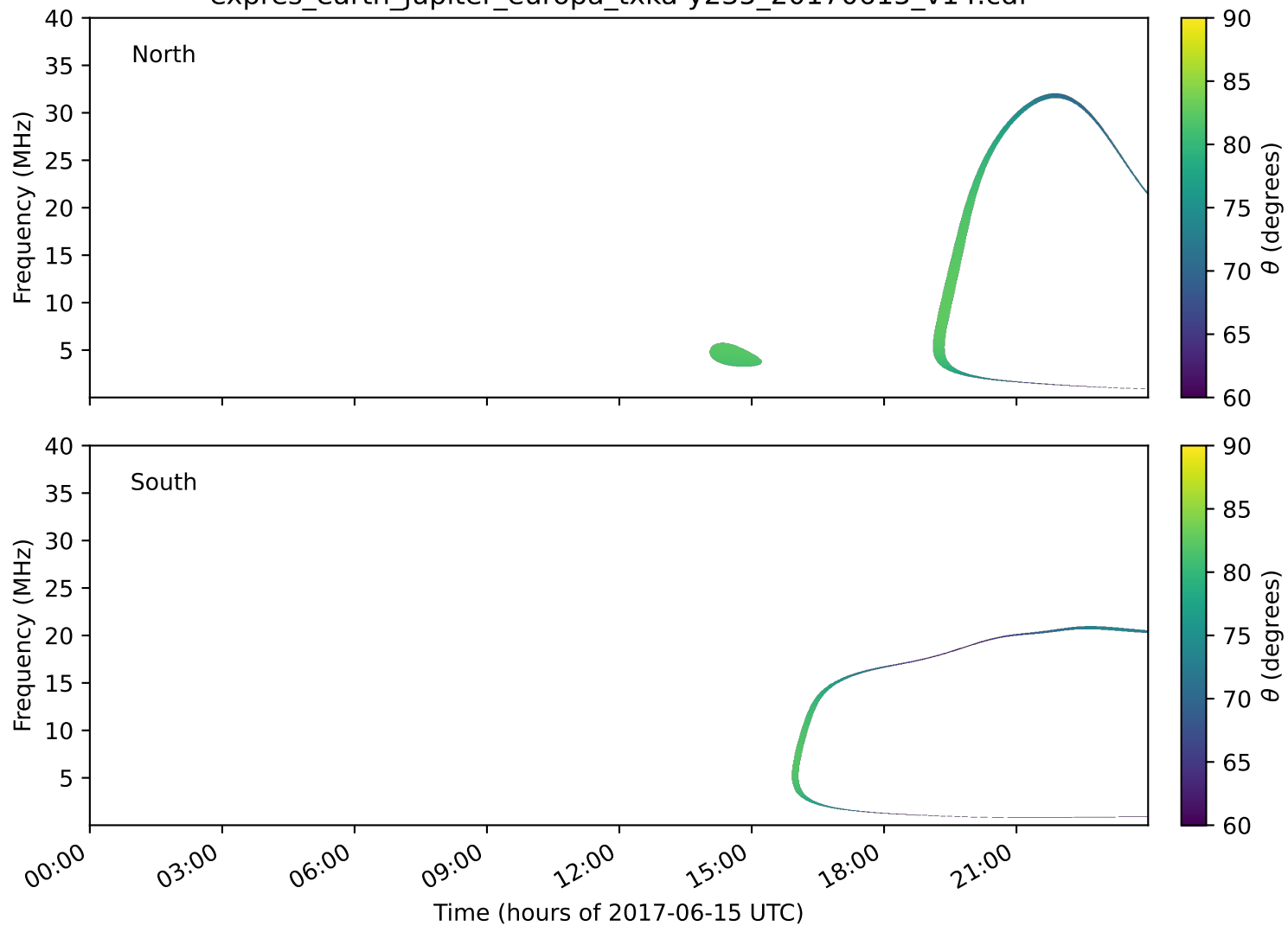
expres_earth_jupiter_europa_txka-y235_20170615_v14.cdf
