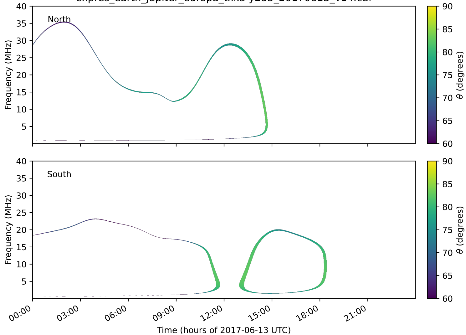
expres_earth_jupiter_europa_txka-y235_20170613_v14.cdf
