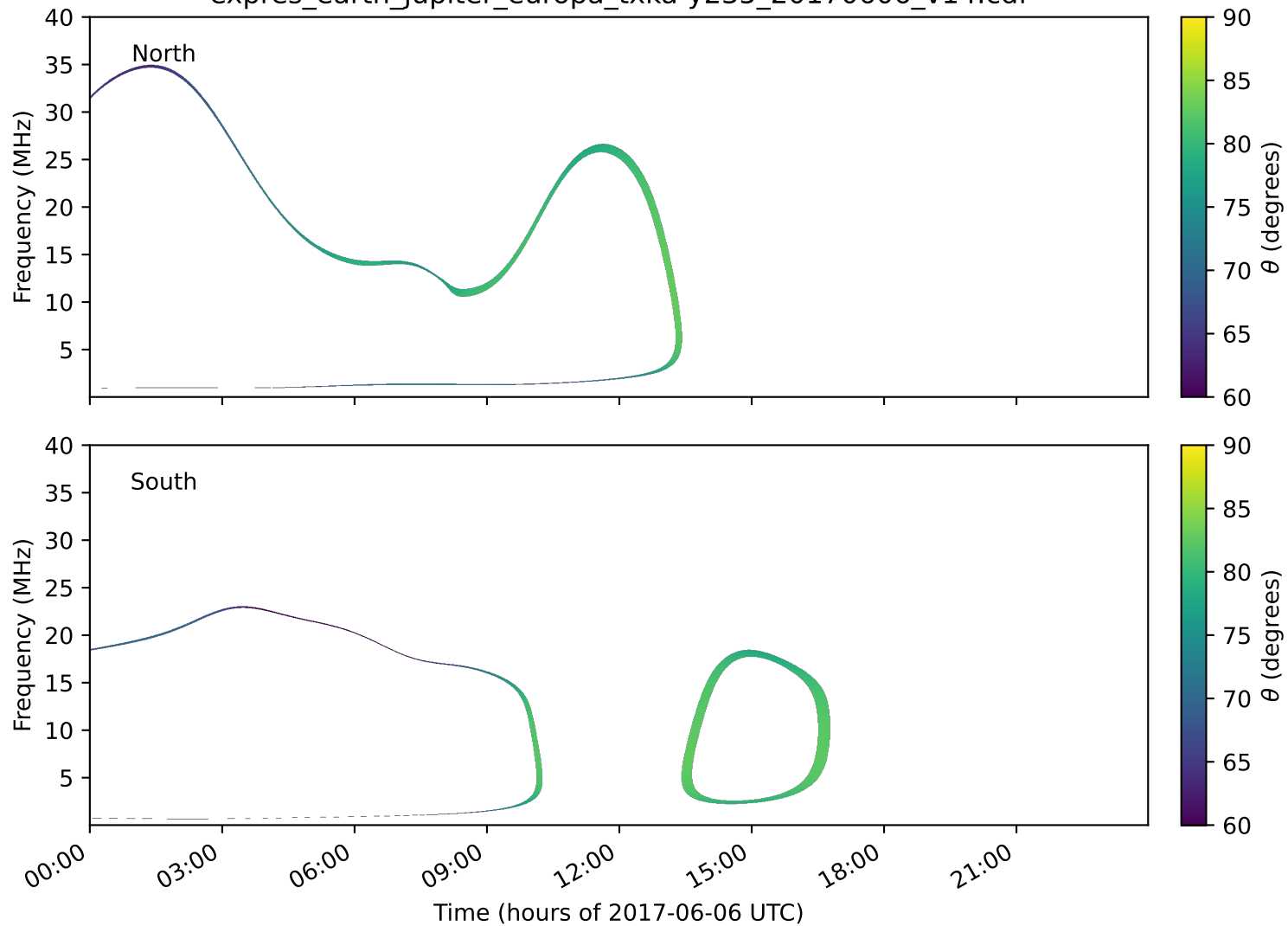
expres_earth_jupiter_europa_txka-y235_20170606_v14.cdf
