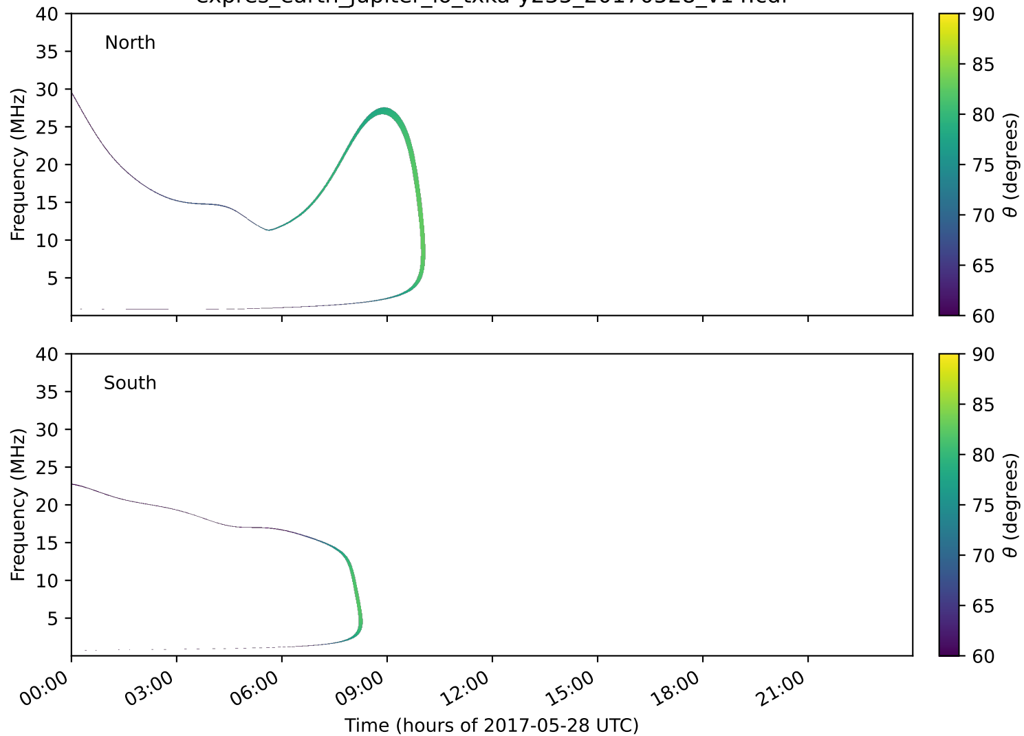
expres_earth_jupiter_io_txka-y235_20170528_v14.cdf
