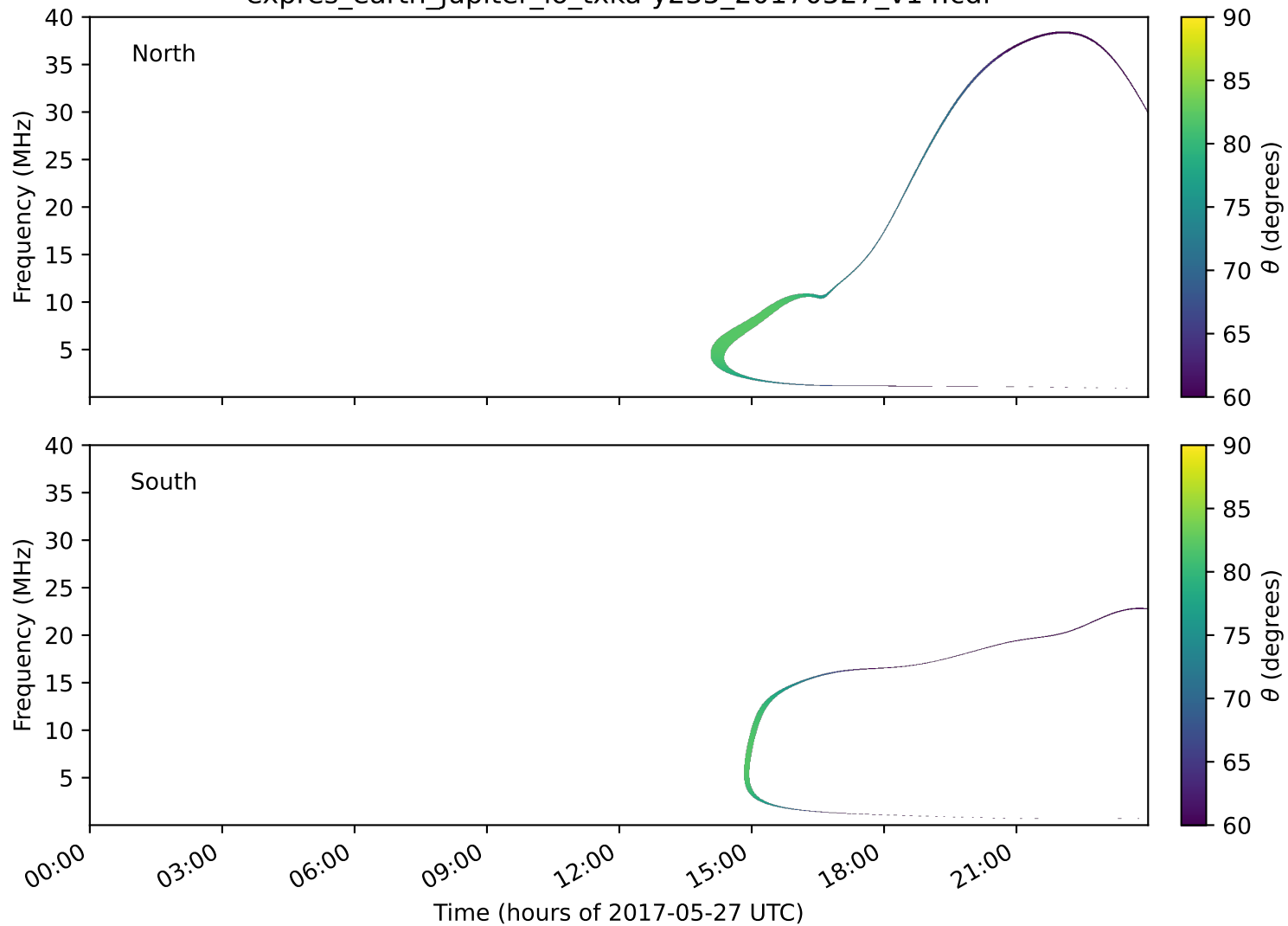
expres_earth_jupiter_io_txka-y235_20170527_v14.cdf
