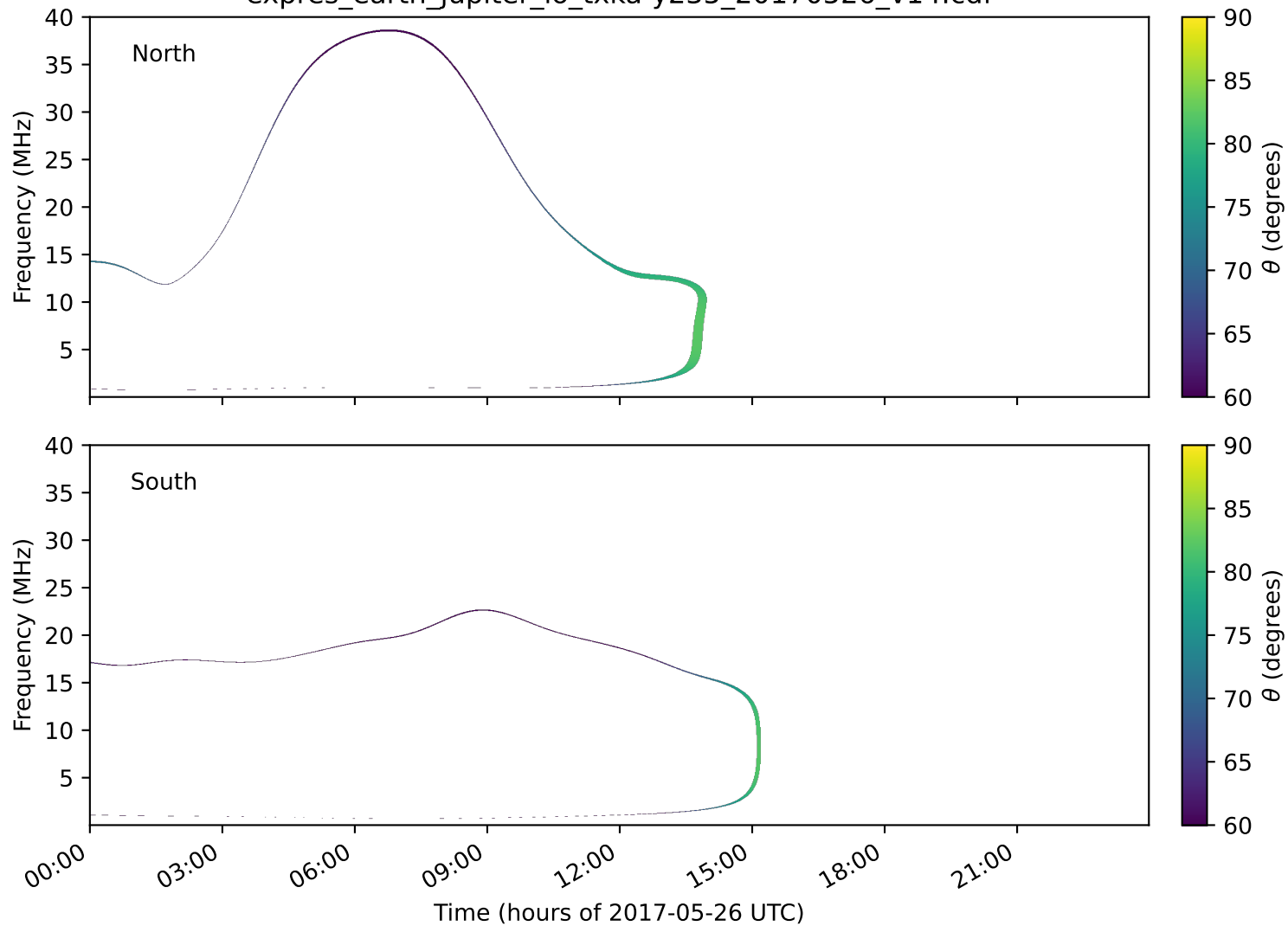
expres_earth_jupiter_io_txka-y235_20170526_v14.cdf
