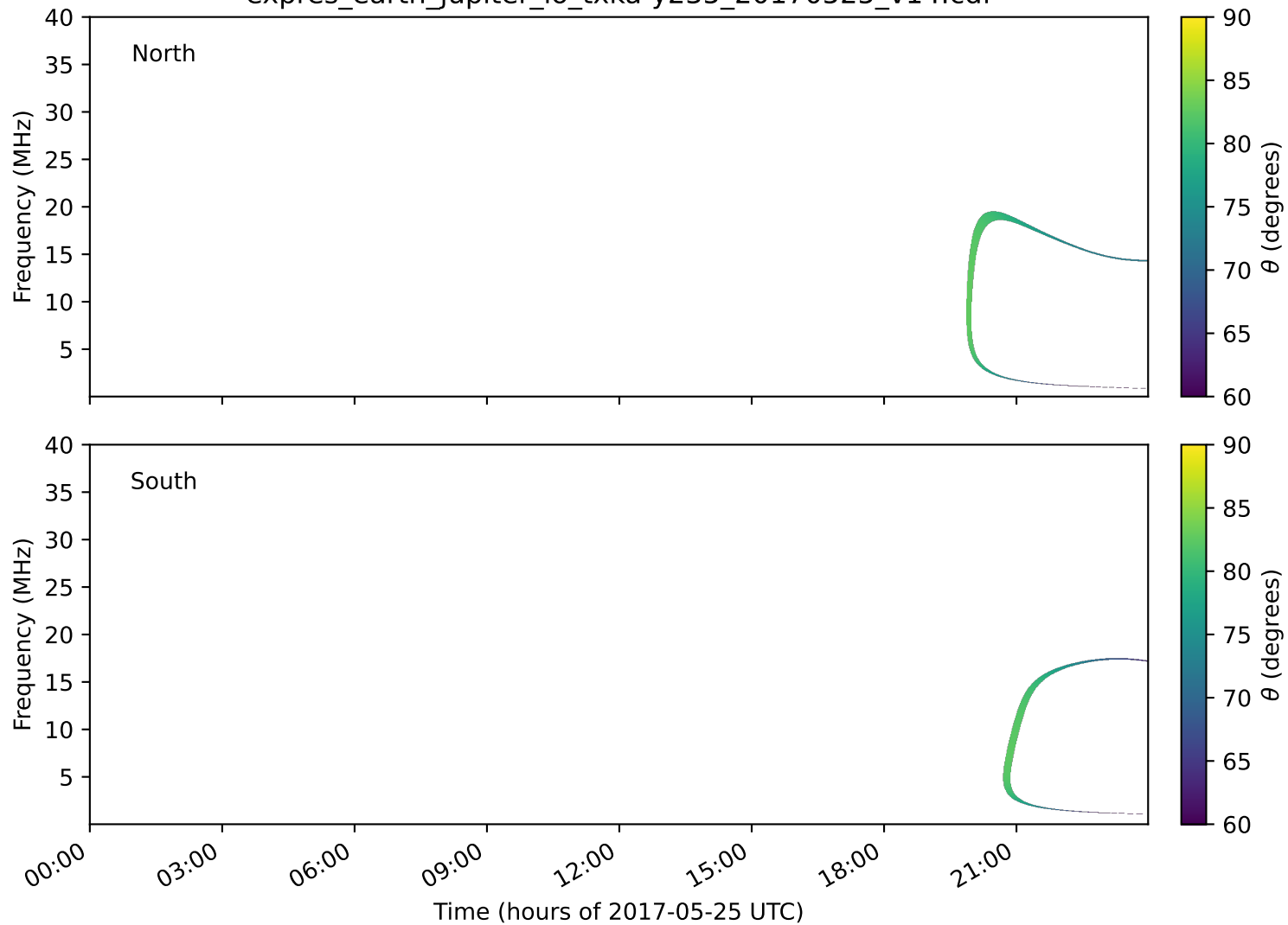
expres_earth_jupiter_io_txka-y235_20170525_v14.cdf
