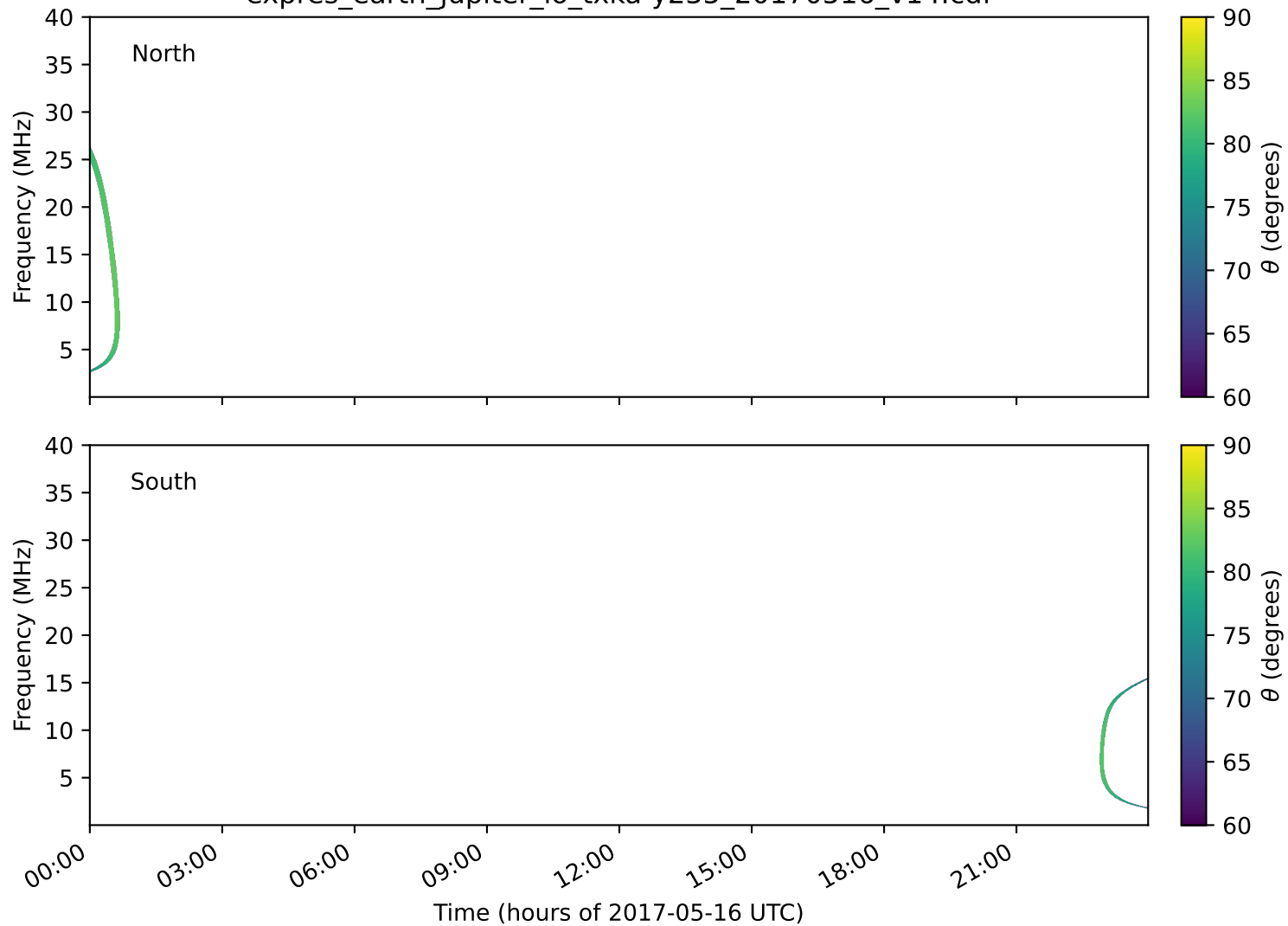
expres_earth_jupiter_io_txka-y235_20170516_v14.cdf
