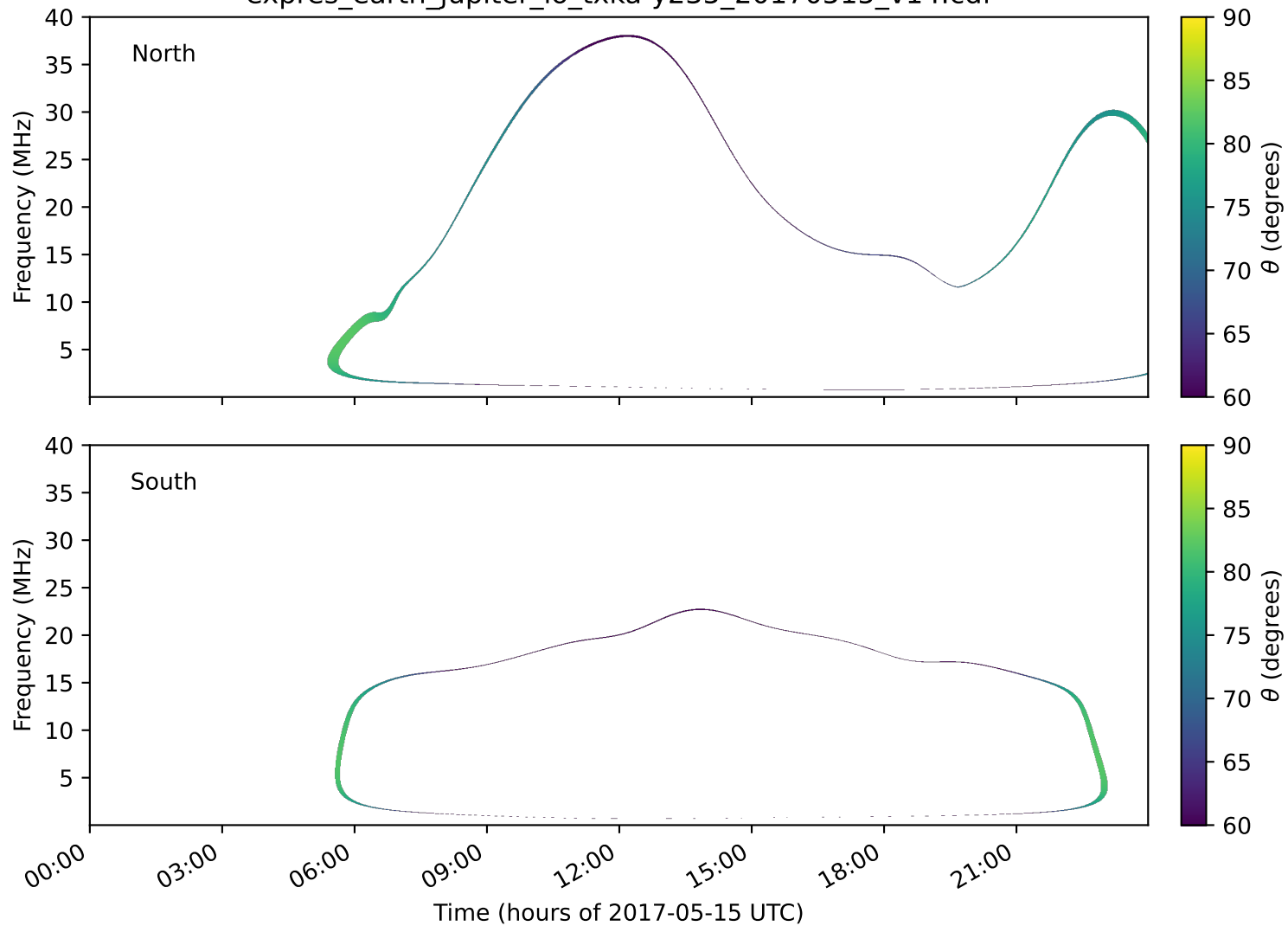
expres_earth_jupiter_io_txka-y235_20170515_v14.cdf
