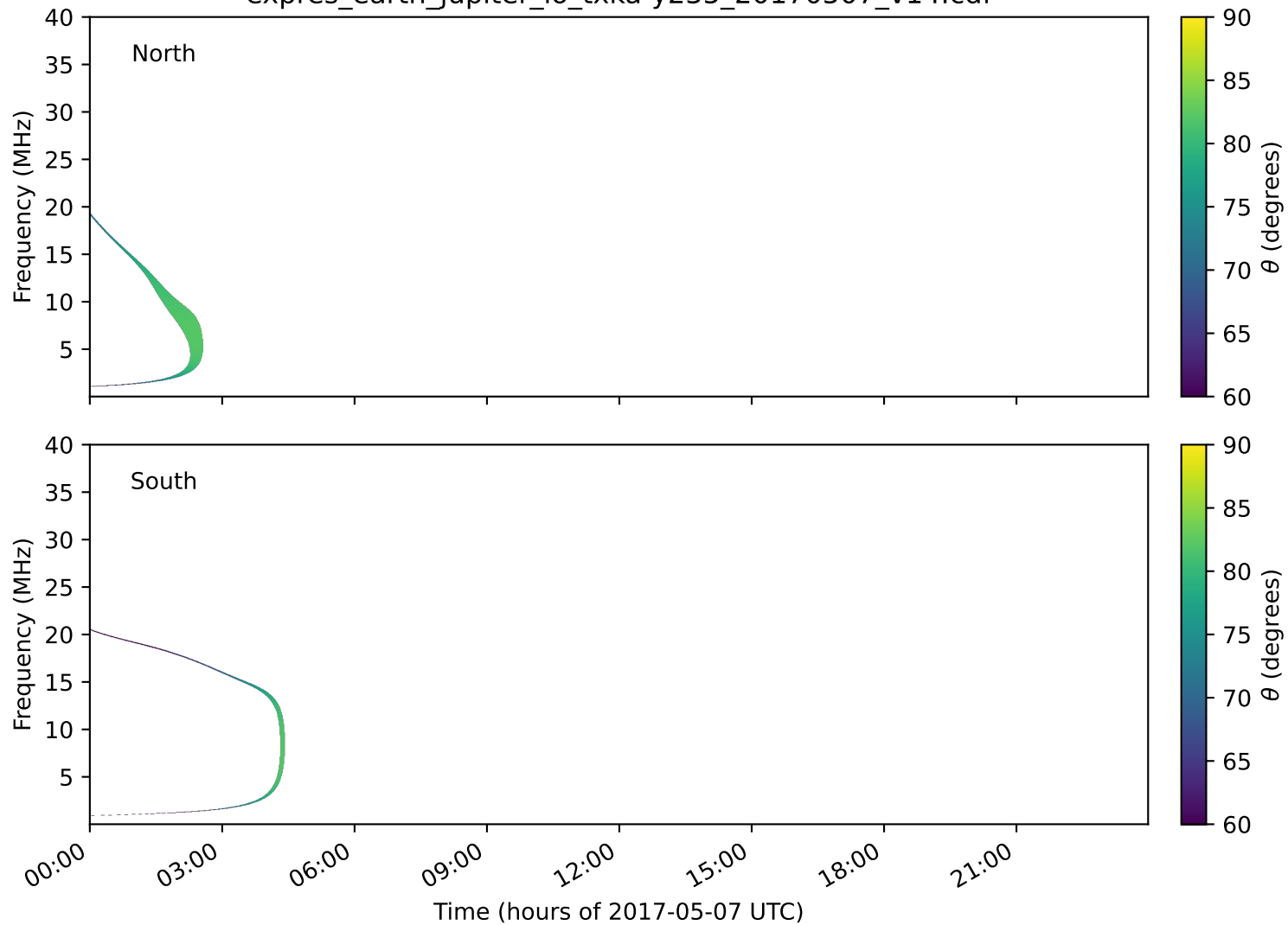
expres_earth_jupiter_io_txka-y235_20170507_v14.cdf
