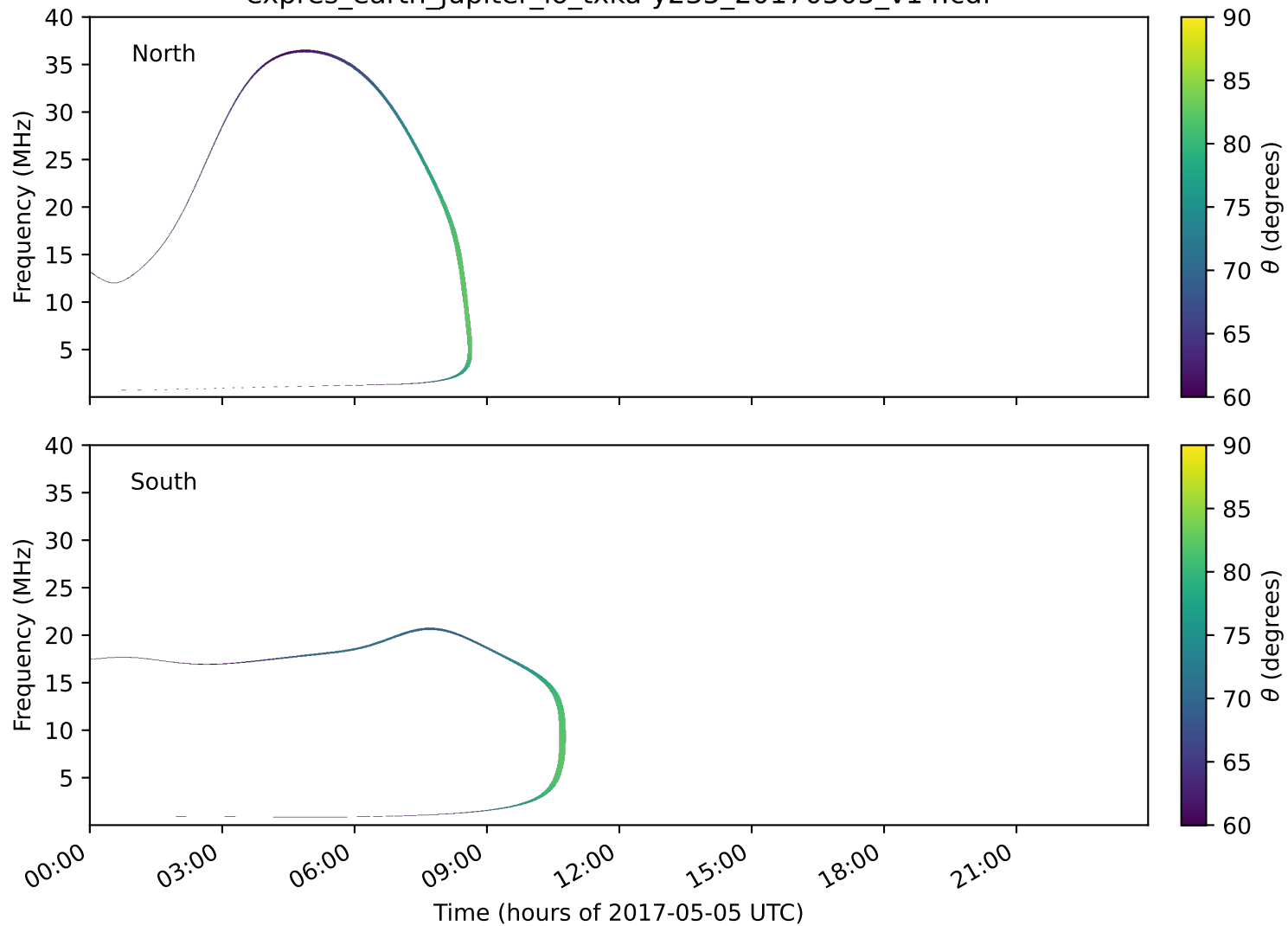
expres_earth_jupiter_io_txka-y235_20170505_v14.cdf
