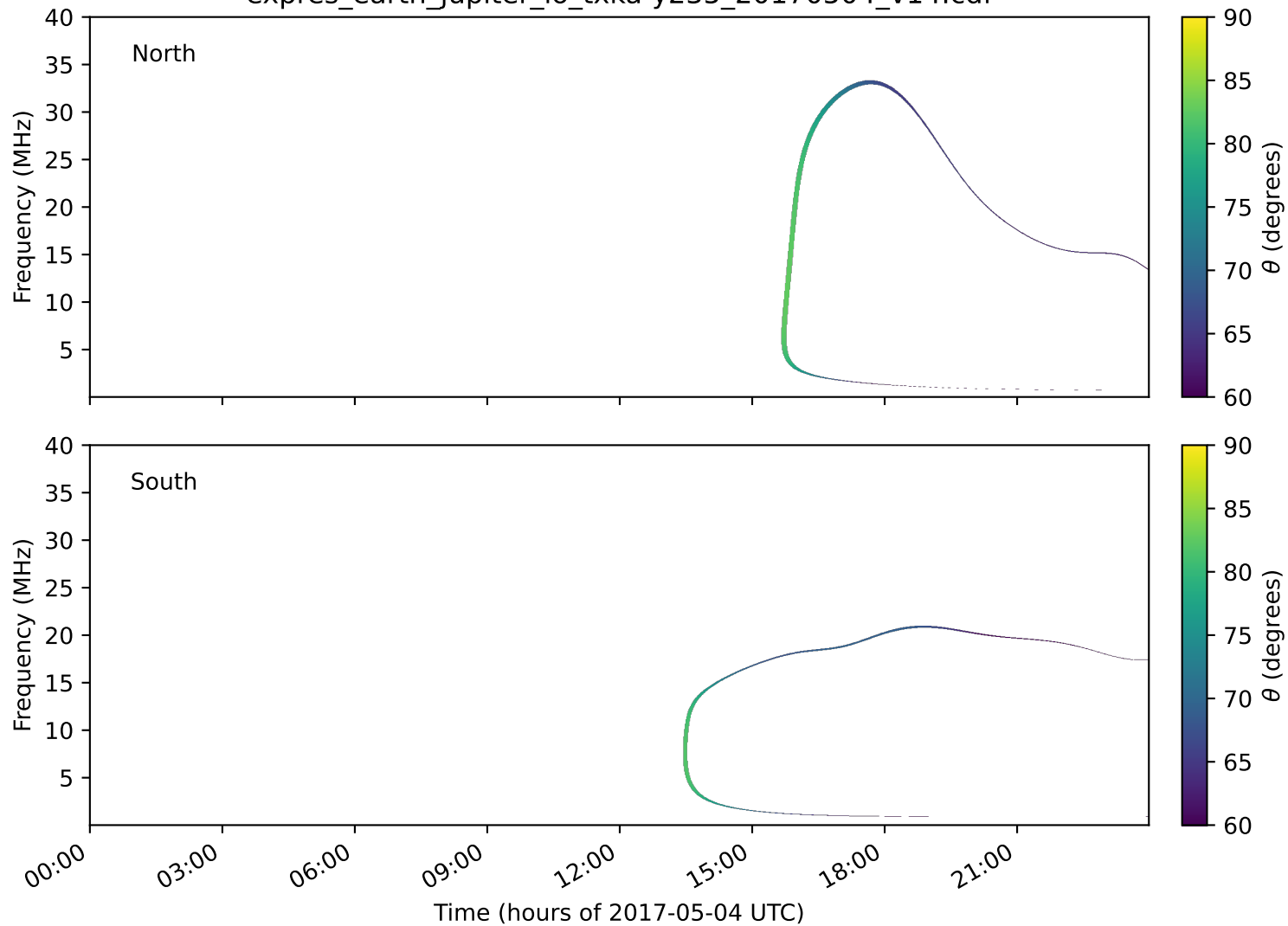
expres_earth_jupiter_io_txka-y235_20170504_v14.cdf
