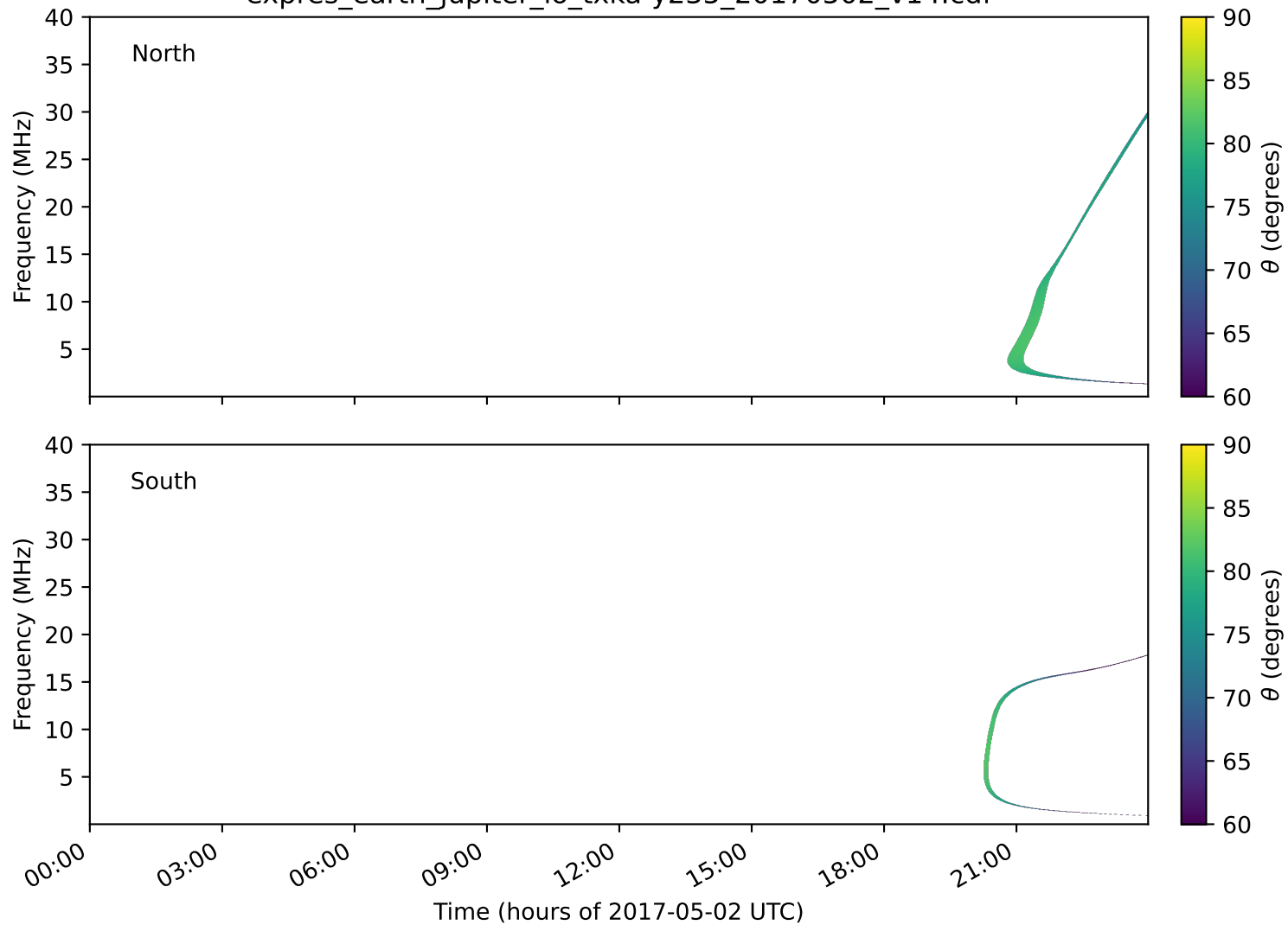
expres_earth_jupiter_io_txka-y235_20170502_v14.cdf
