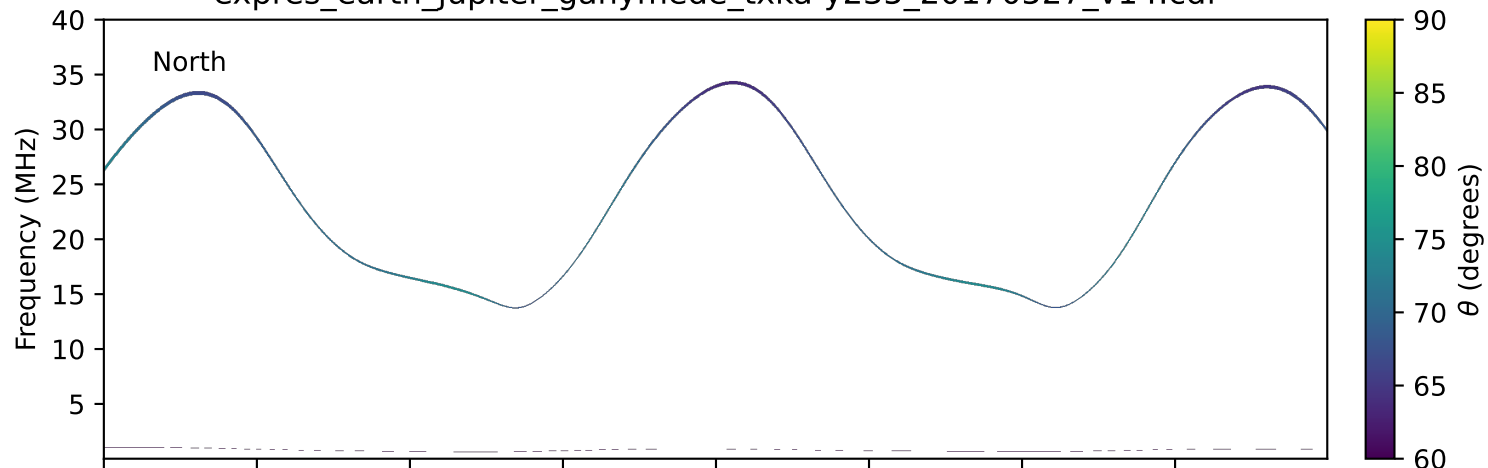
expres_earth_jupiter_ganymede_txka-y235_20170527_v14.cdf
