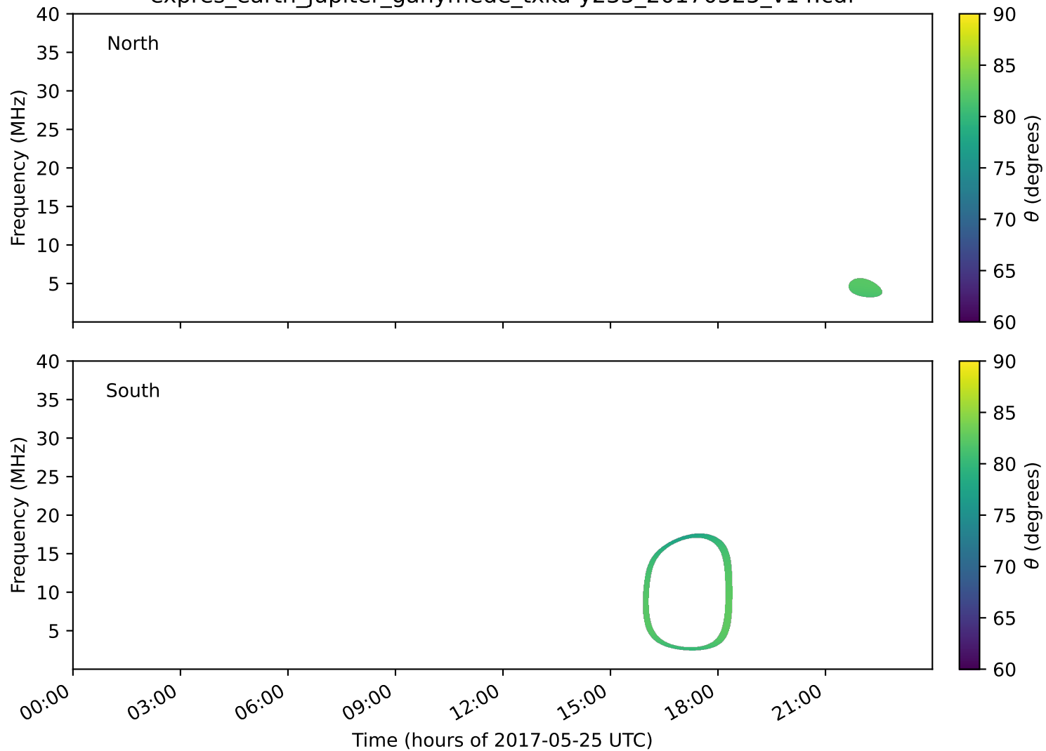
expres_earth_jupiter_ganymede_txka-y235_20170525_v14.cdf
