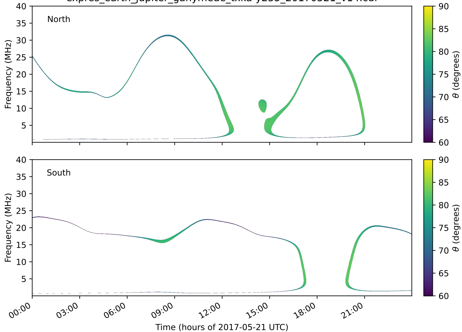
expres_earth_jupiter_ganymede_txka-y235_20170521_v14.cdf
